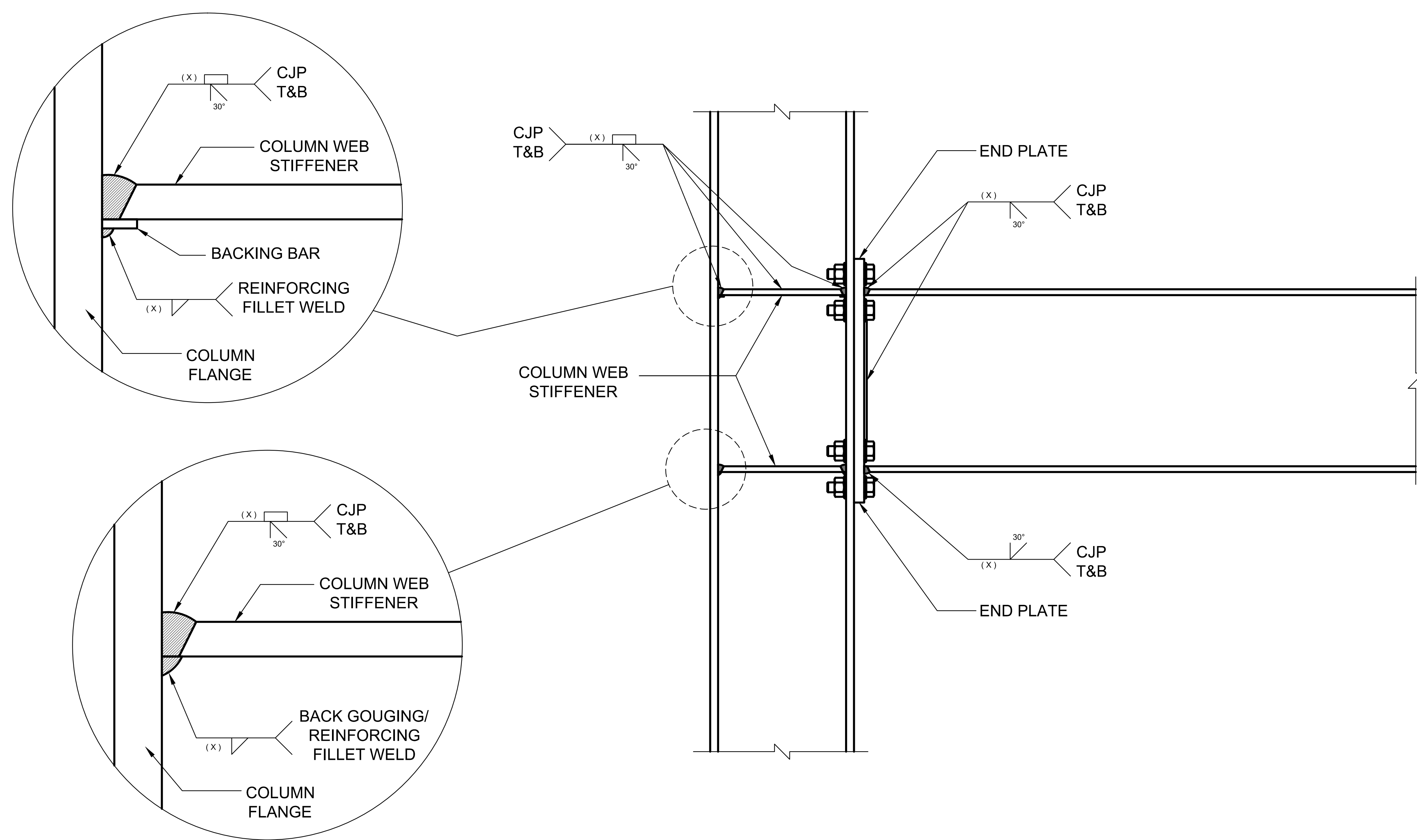
Four-Bolt Unstiffened (4E)
