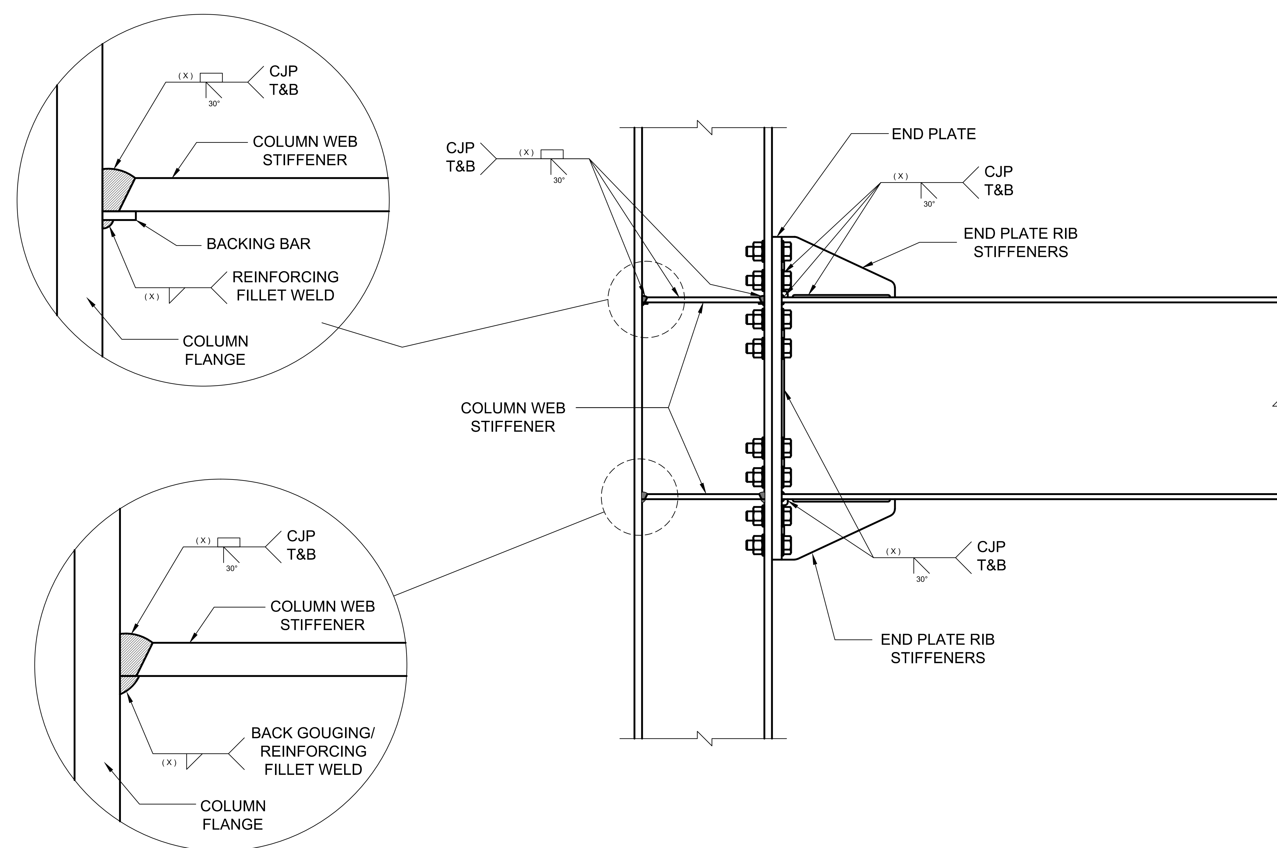
Eight-Bolt Stiffened (8ES)
